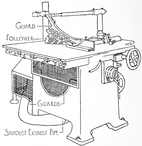
FIG. 158. SAW GUARDS.
